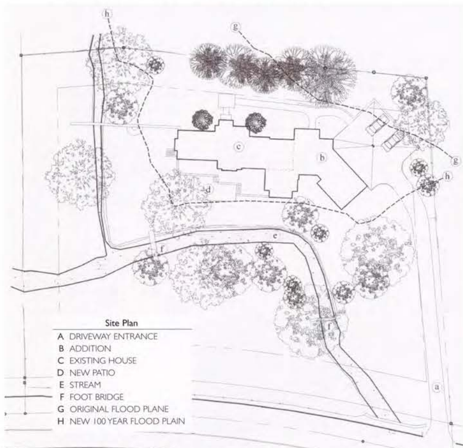
The site plan illustrates how the angled addition responds to the stream and flood plain. New footbridges link the grounds of the main house to the wooded landscape opposite the stream.
